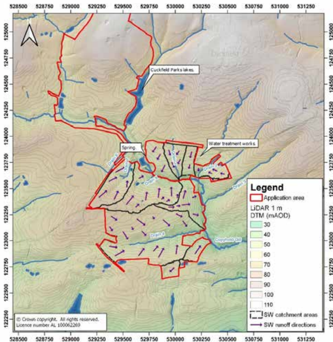
Figure 2-3 Site topography and current runoff regime in development area
