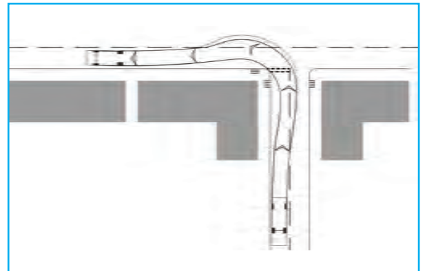
Despite the small corner radius, with sufficient carriageway width (X) a long vehicle can still negotiate a junction.
