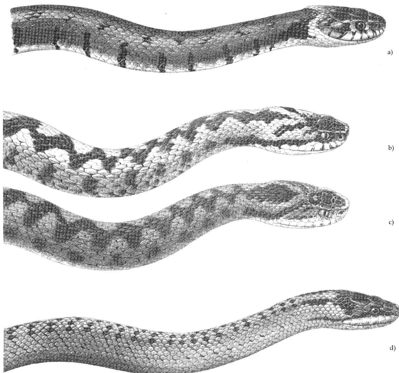
Figure 15 a) Grass snake; b) male adder; c) female adder; and d) smooth snake. Note the typical markings, the collar of the grass snake and the eye stripe and dark crown of the smooth snake.
