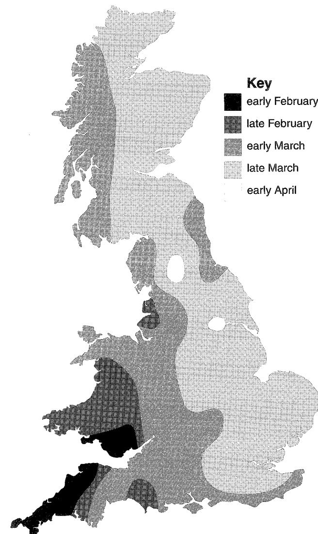
Figure 2 Spawning dates of the common frog (adapted from: Cooke 1976).
